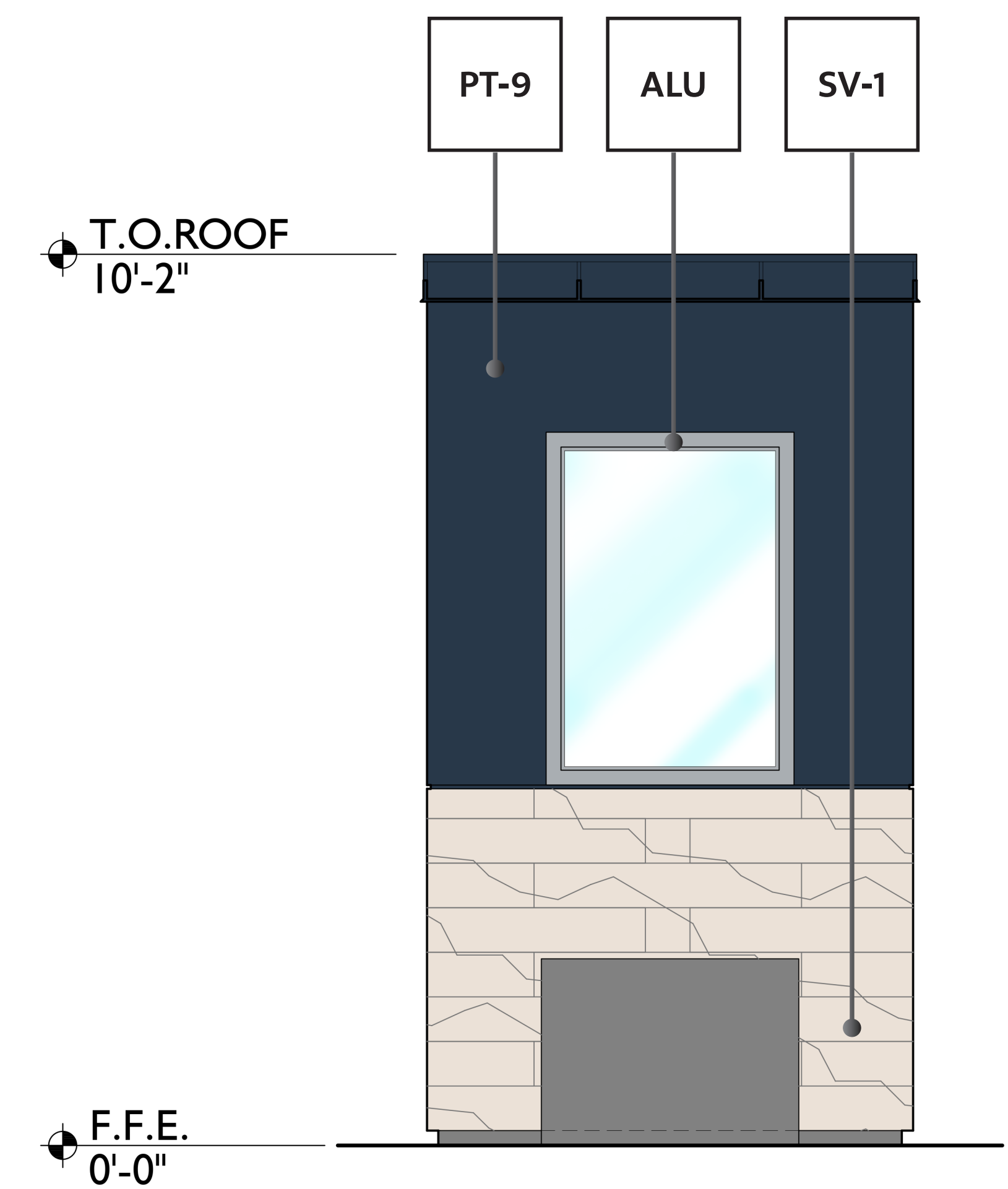
13 ATTENDANT SHELTER READ ELEVATION
