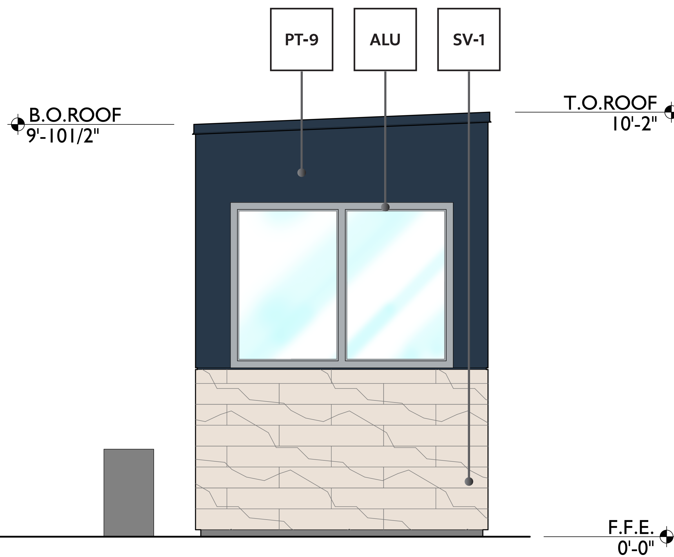
12 ATTENDANT SHELTER SIDE ELEVATION
