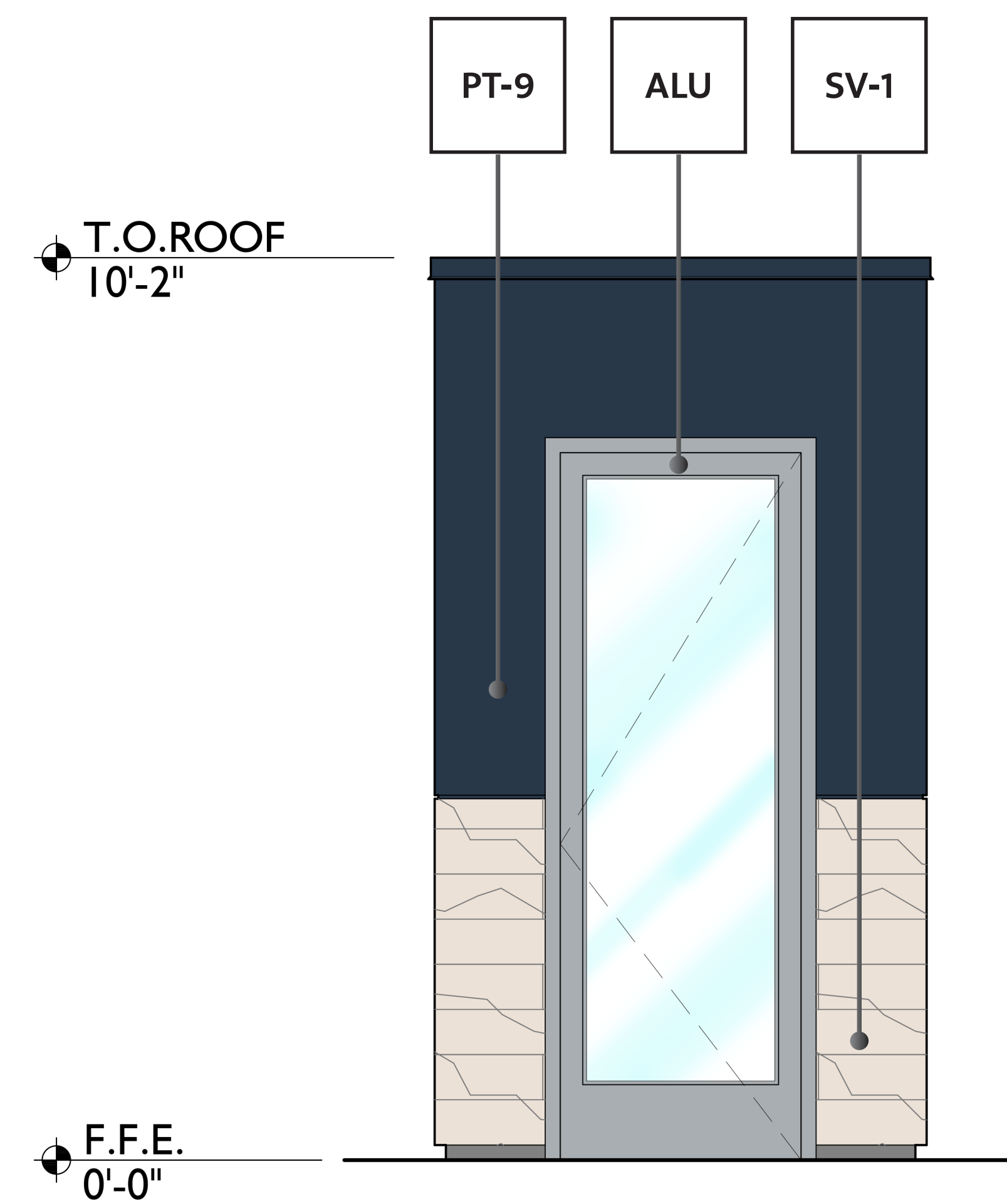
11 ATTENDANT SHELTER FRONT ELEVATION
