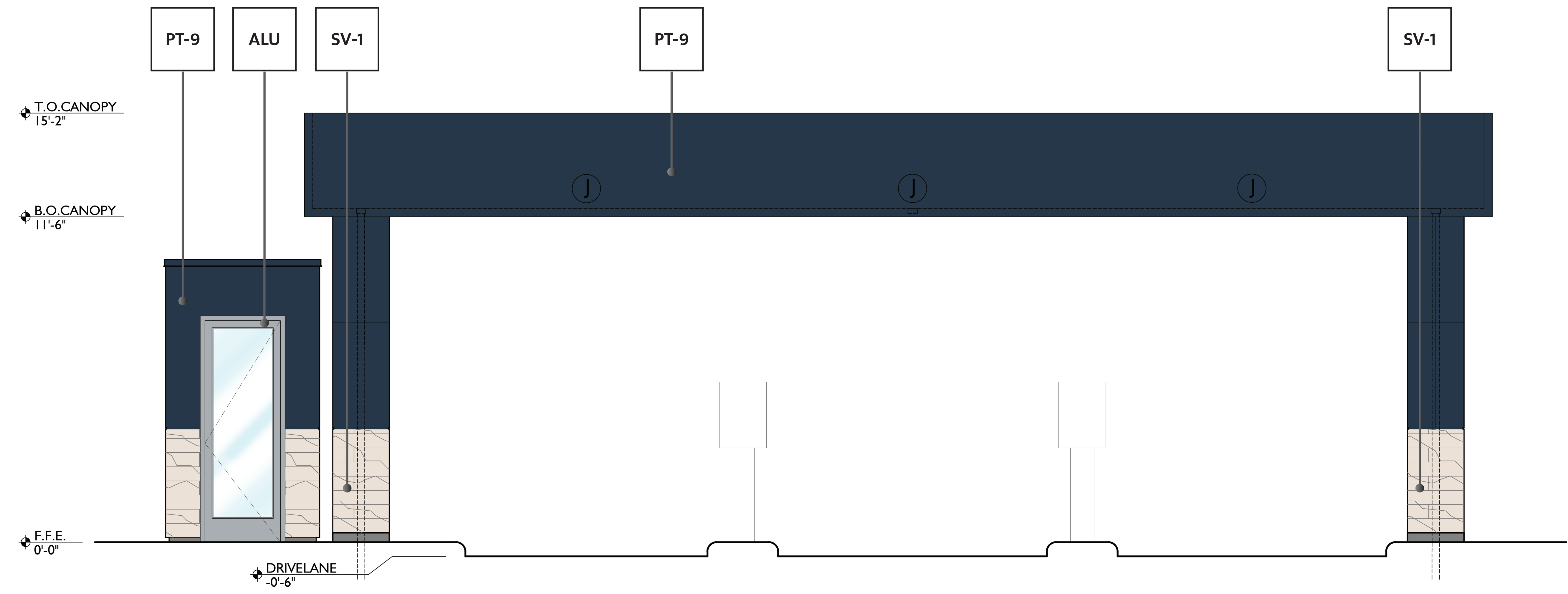
15 POS CANOPY FRONT ELEVATION 1/2" = 1'
