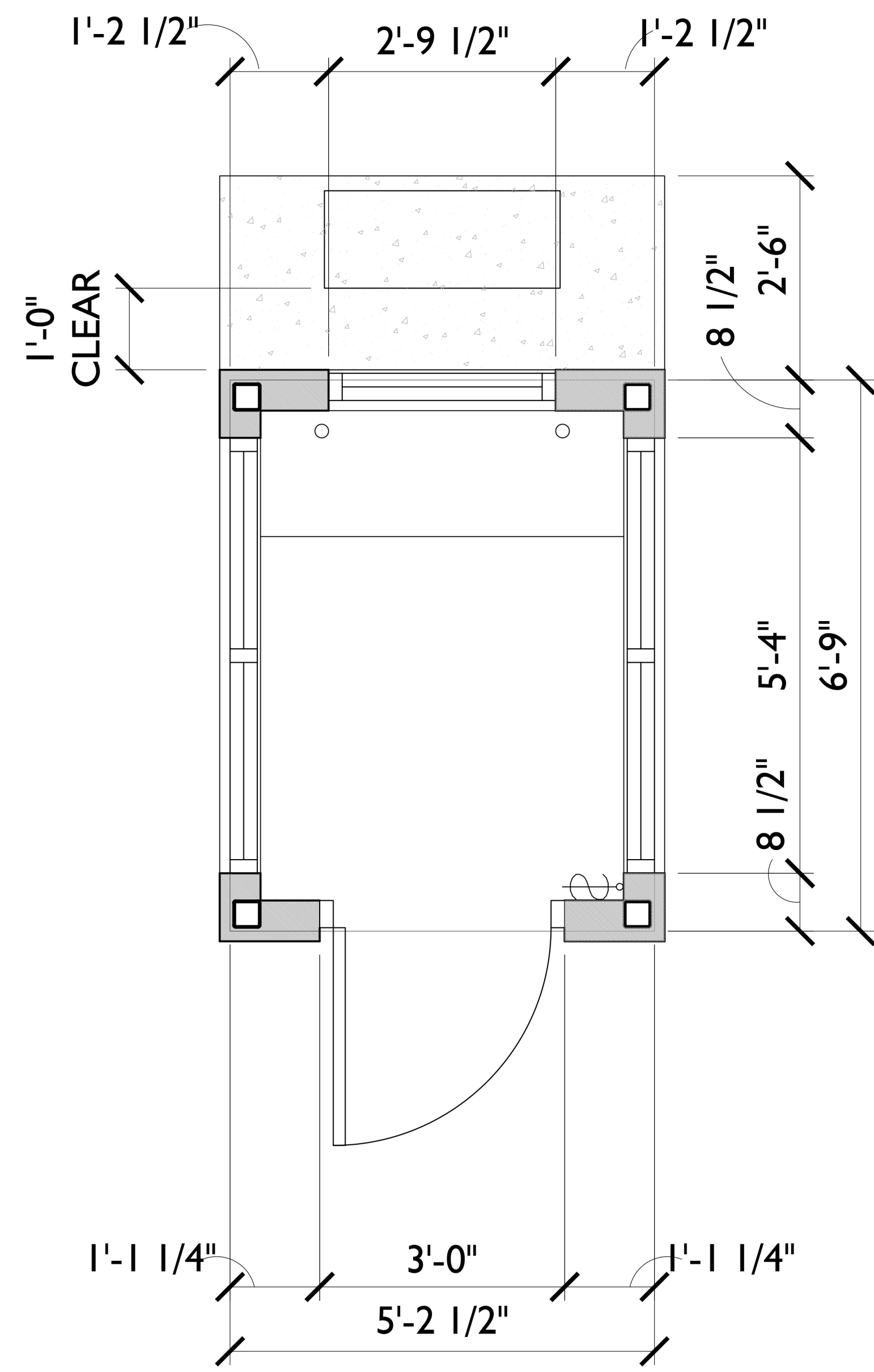
9 ATTENDANT SHELTER PLAN
