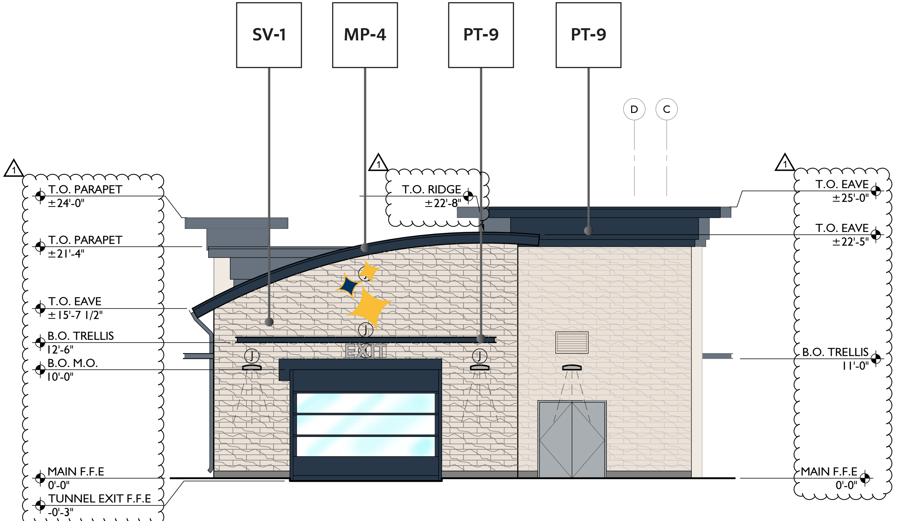
NORTH ELEVATION: CAR WASH TUNNEL EXIT
