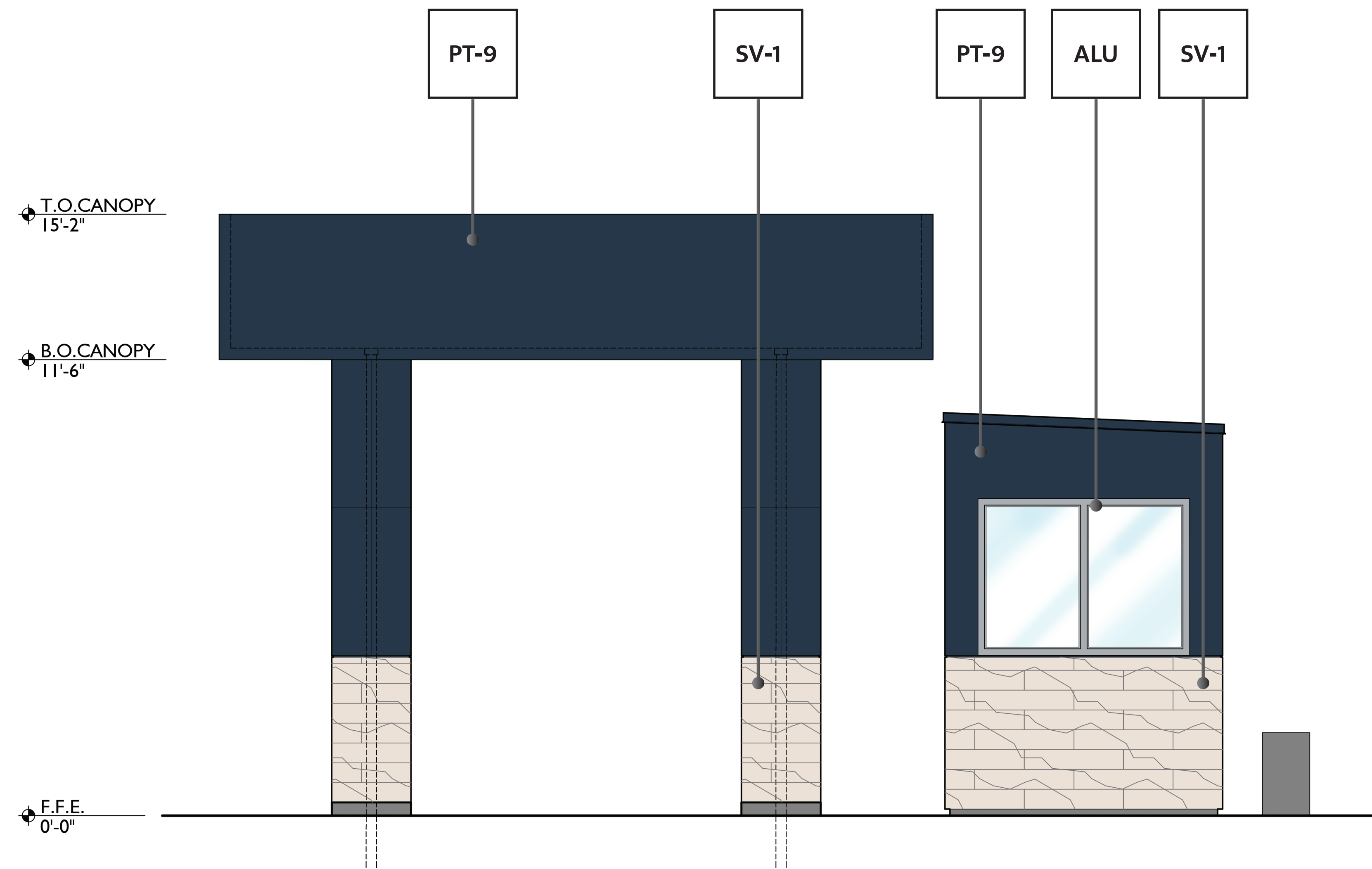
14 POS CANOPY SIDE ELEVATION 1/2" = 1'
