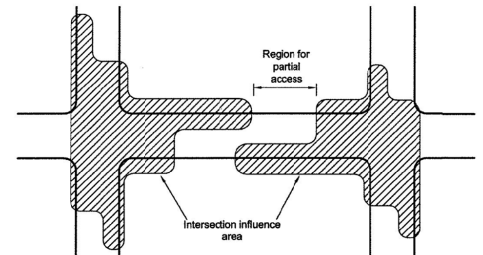
Figure 44-3: Partial Access Between Functional Areas 2 .
