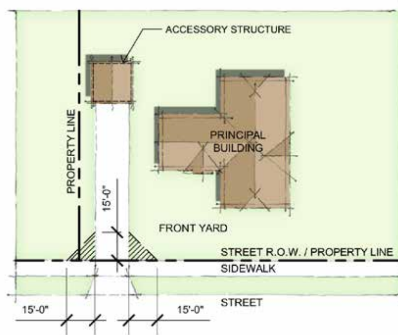
Figure 49-2: Driveway Vision Clearance
