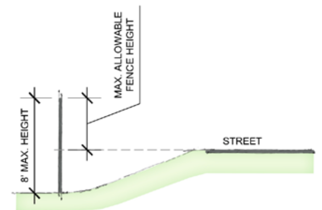
Figure 98-1: Below Street-Grade Fence
