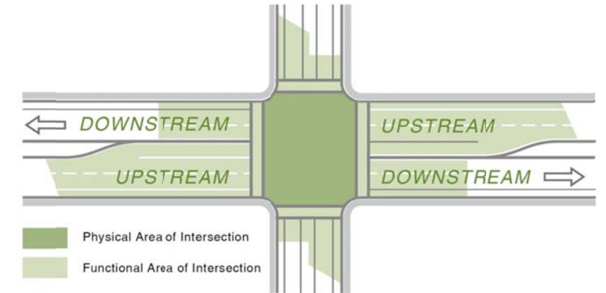
Figure 44-2: Comparison of the Intersection Physical and Functional Area 1 .
